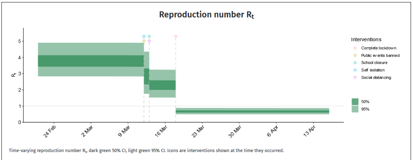
Figure 8. Relation of different non-pharmaceutical interventions to R_t Example from Denmark (Flaxman et al., 2020)
