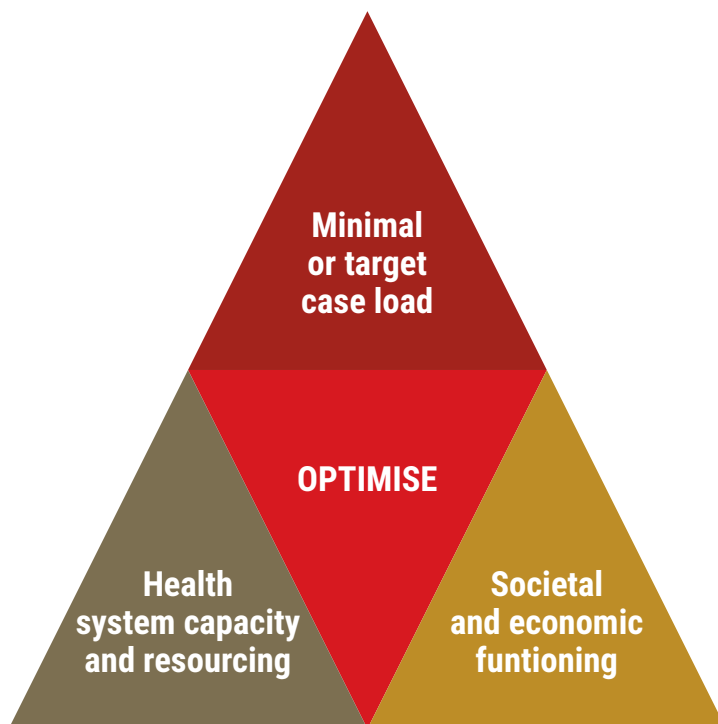
Figure 1. Controlled adaptation as an optimisation problem (and solution)
