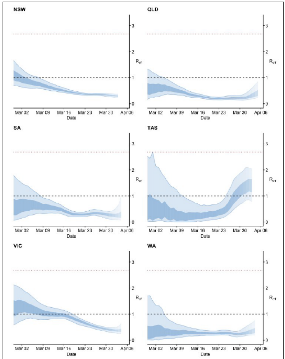
Figure 4. Time-varying estimate of the effective reproduction number of COVID-19
