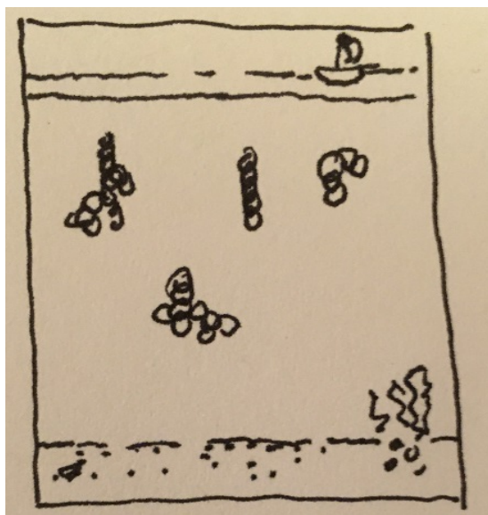
Figure 2. Disease in Transmission Chains
